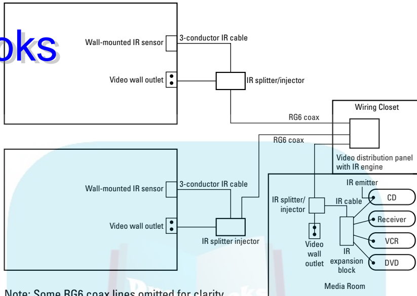
Figure 20-1: Piggy-backing IR signals on a coaxial network.
